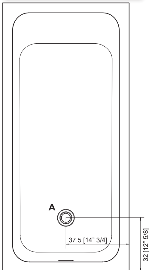
MODUL 159 x 75 [62 5/8" x 29 4/8"]
