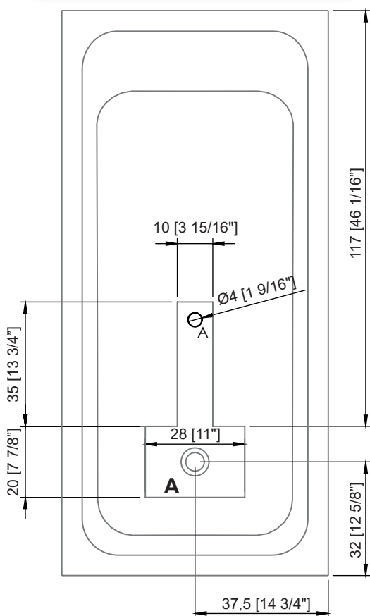
MODUL 159 x 75 [62 5/8" x 29 4/8"]
