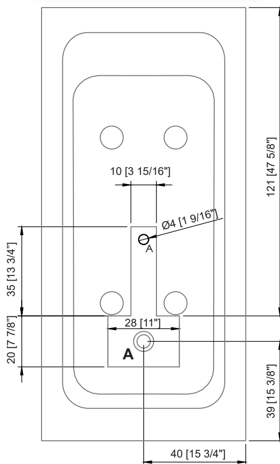
MODUL 170 x 80 [66 7/8" x 31 4/8"]
